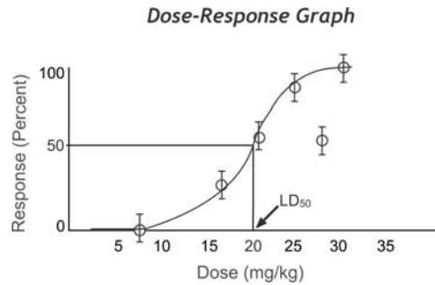
FIGURE 1.4 Sigmoid curve typical of an LD 50 test (Courtesy of National Library of Medicine. Based on original from http://aquaticpath.umd.edu/appliedtox/images=toxtutor/chart-5.gif . Drawn by Patient Education Institute).
